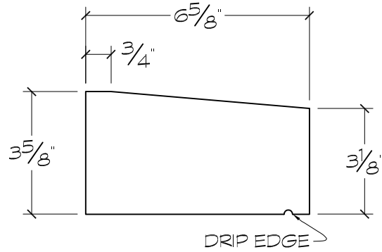
CROSS SECTION
